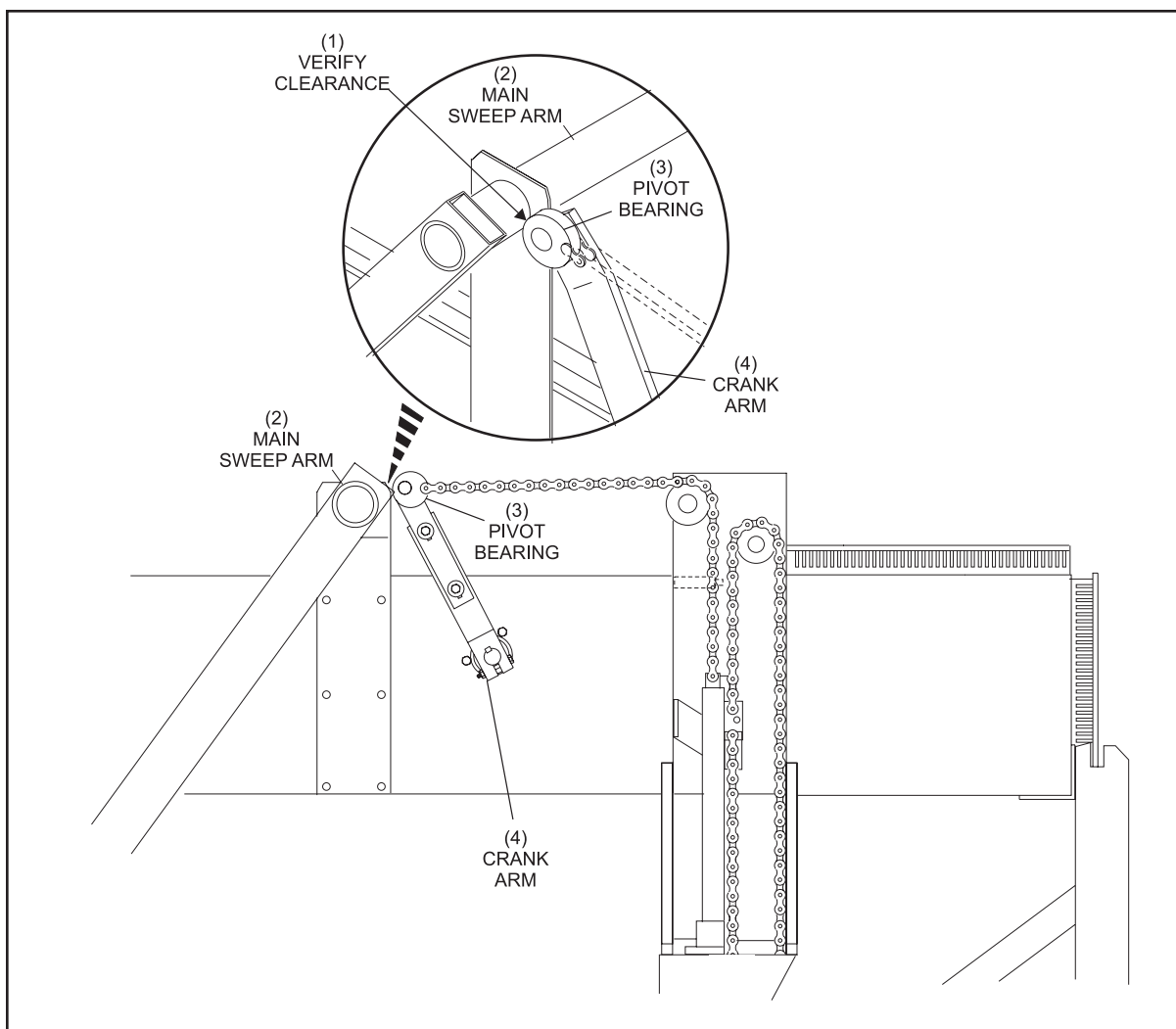
Figure 5-36. Check Pivot Bearing Clearance
