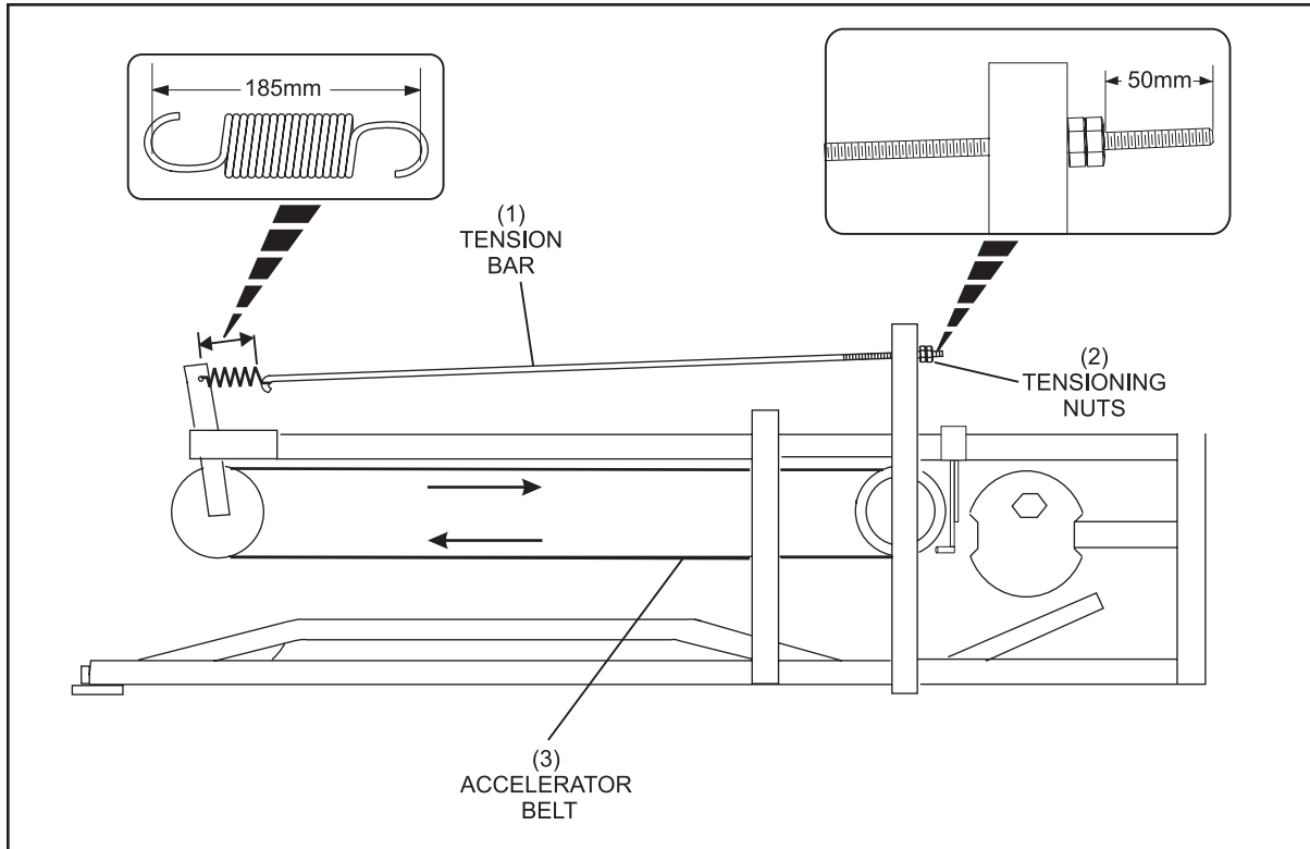
Figure 5-14. Ball Accelerator Flat Belt Tension Adjustment.
