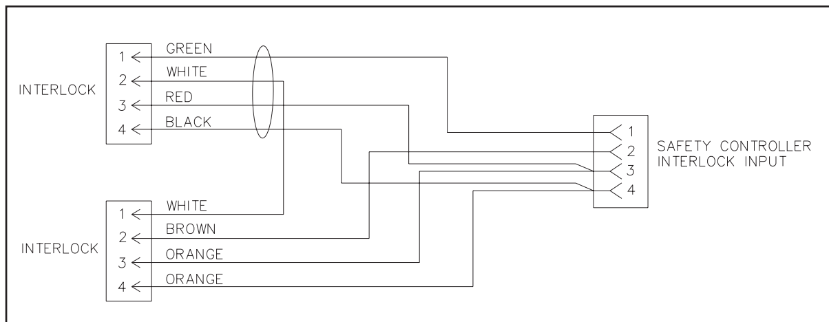
47-142878-000 - Interlock "Y" Cable for Odd and Separated Lane Pairs
