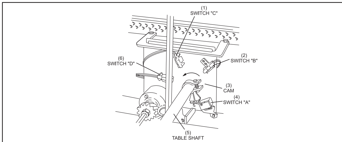
Figure 1-31. Switch Cluster Assembly.
