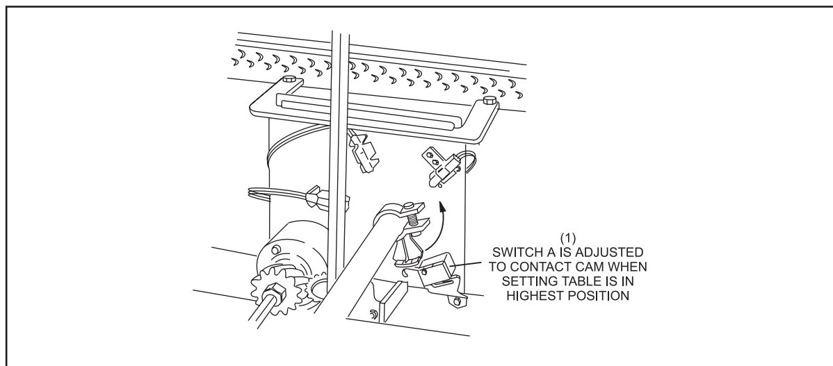
Figure 5-62. Adjusting Switch “A.”
