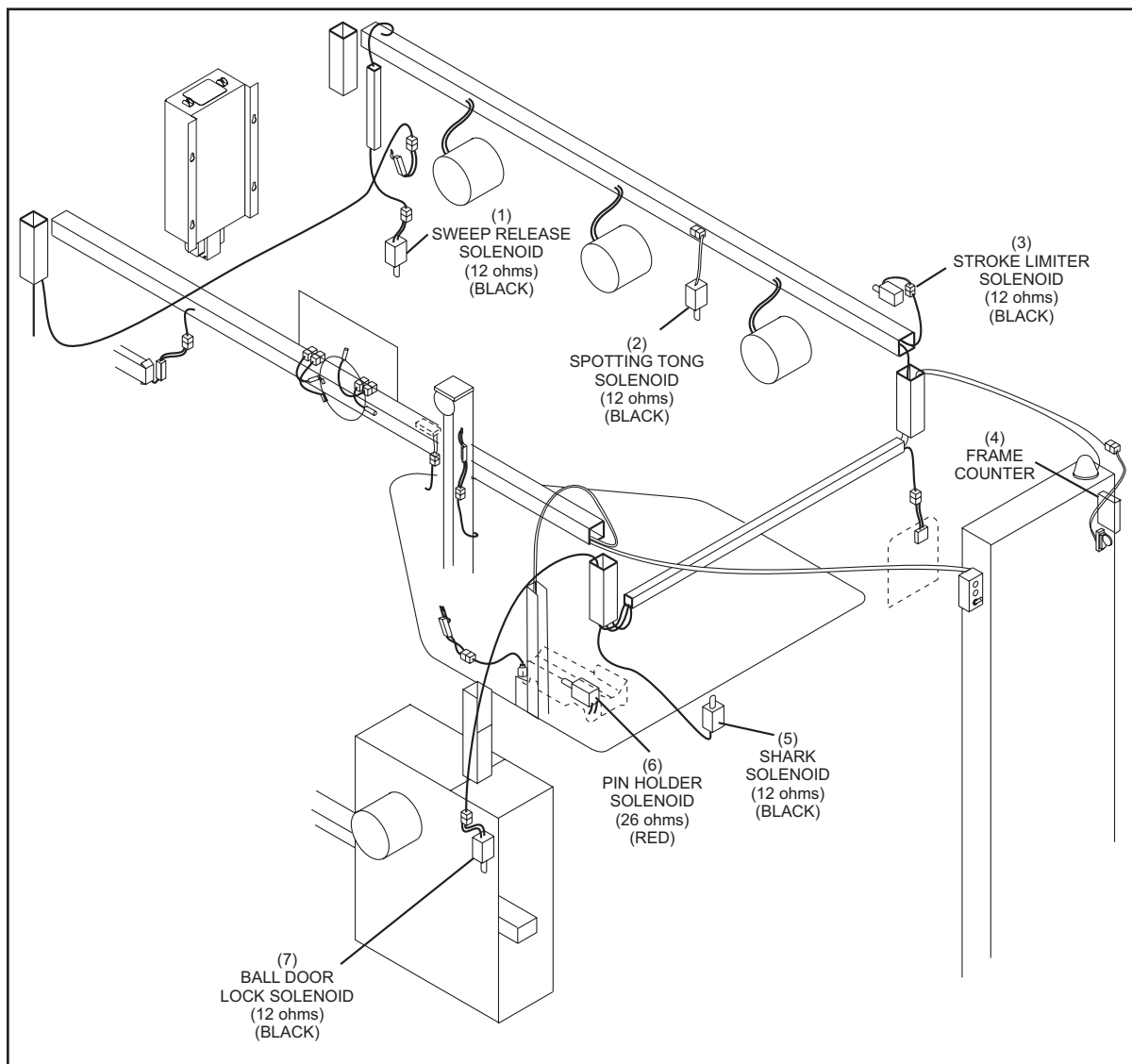
Figure 2-15. Solenoids
