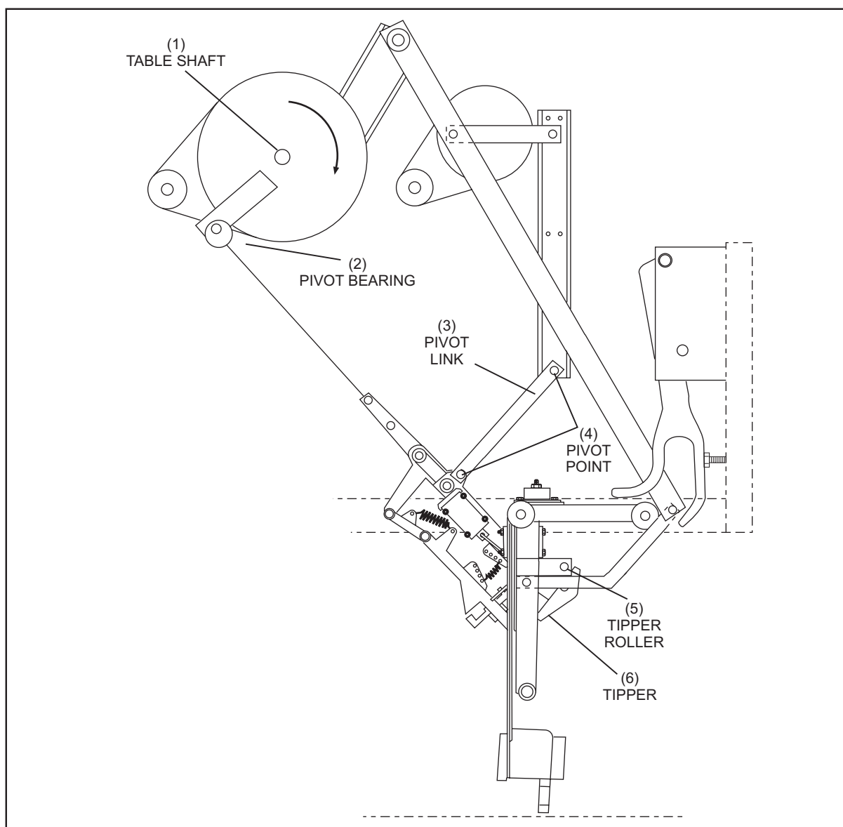
Figure 1-28. Raising the Sweep (CW).
