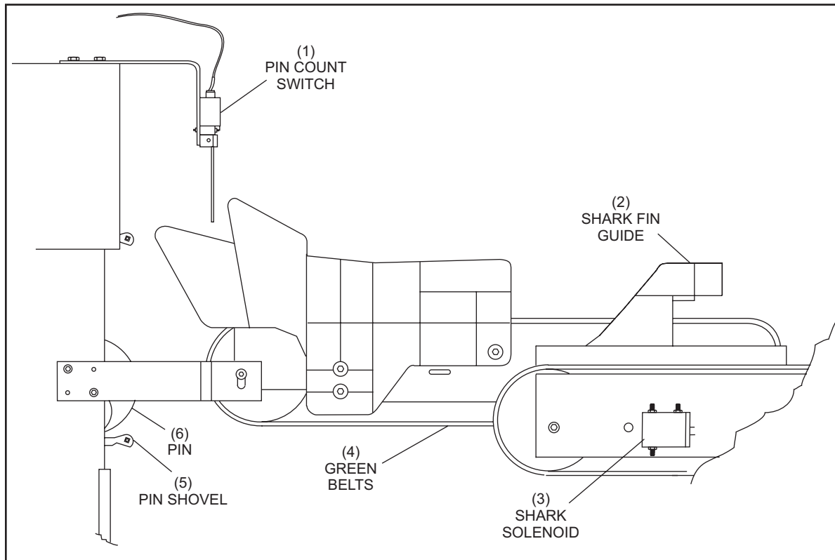
Figure 2-21. Shark Solenoid
