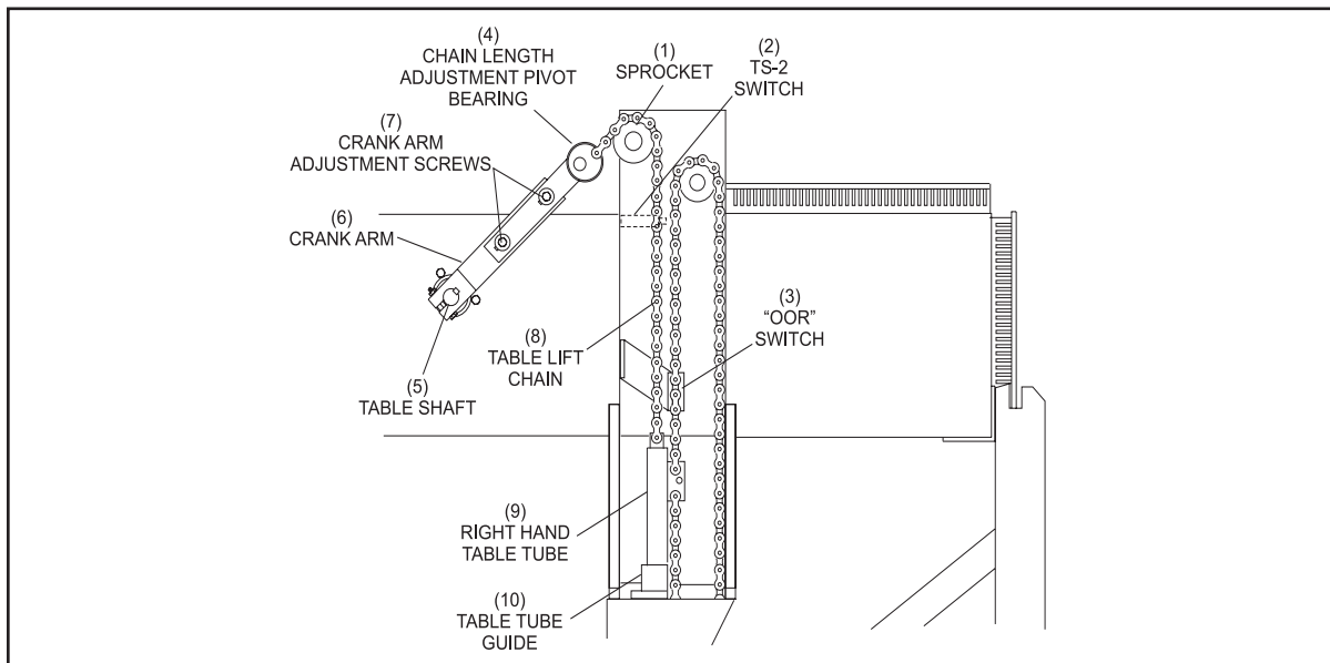
Figure 1-16. Right-Hand Table Rack
