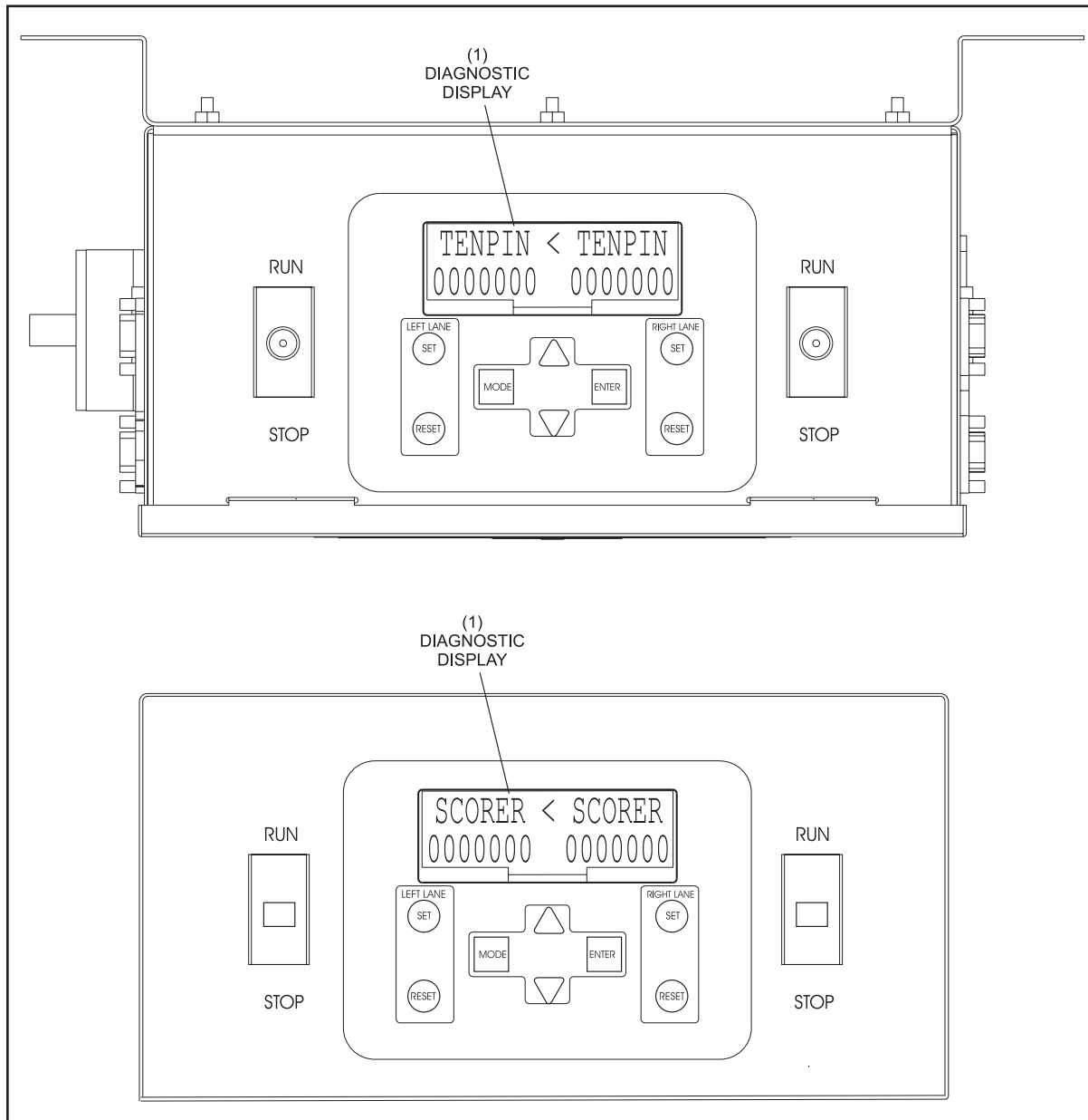
Figure 6-1. Top of Nexgen Controller / Mechanic's Remote Display.
