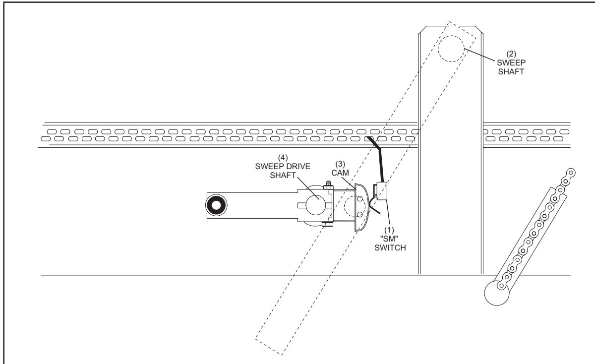
Figure 2-10. SM Switch
