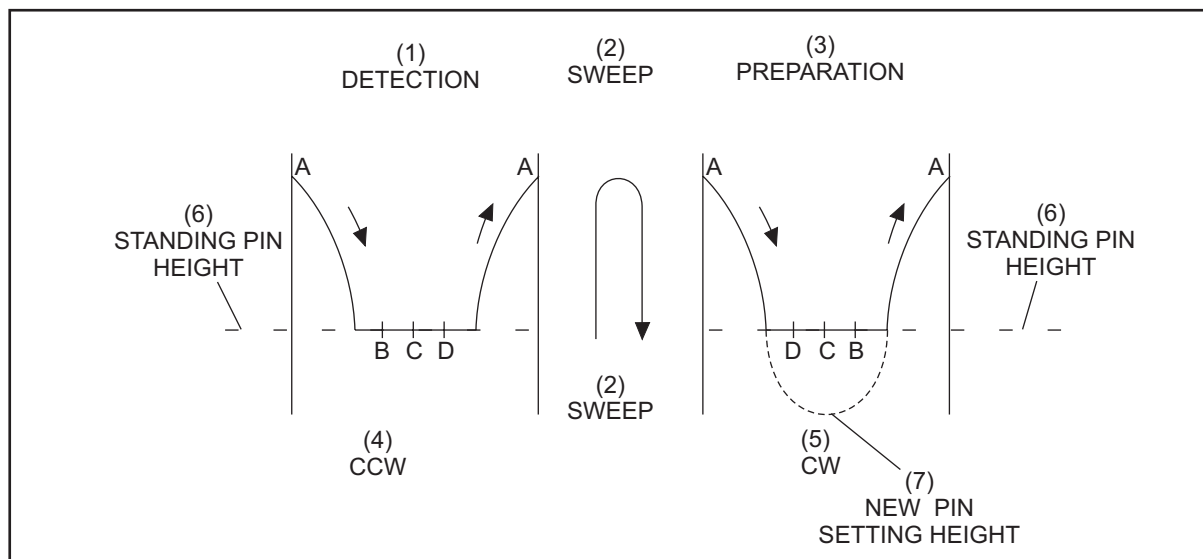
Figure 4-1. Cycle Segments
