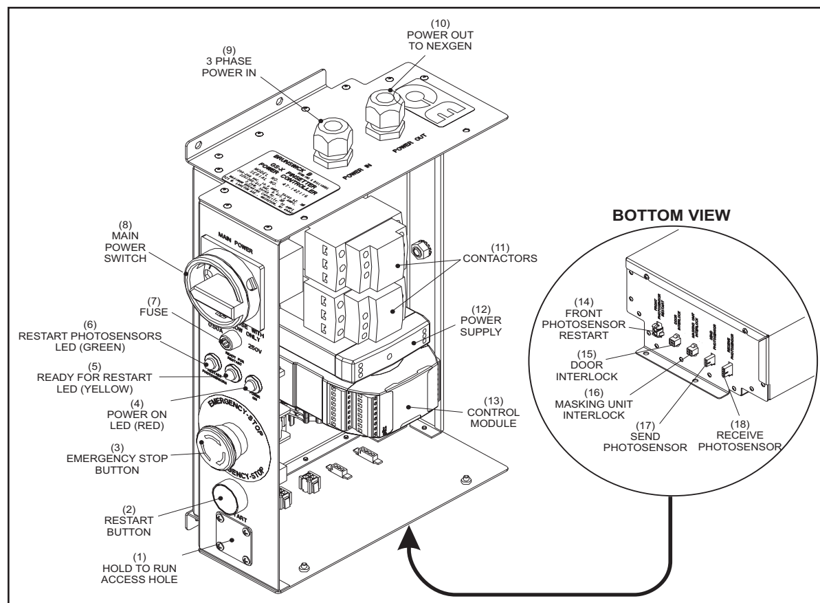
Figure 3-14. Safety Power Controller - Version III
