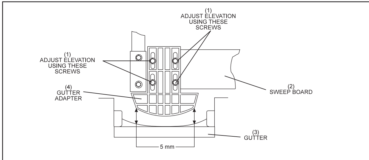
Figure 5-54. Sweep Board Gutter Adapter Adjustment.
