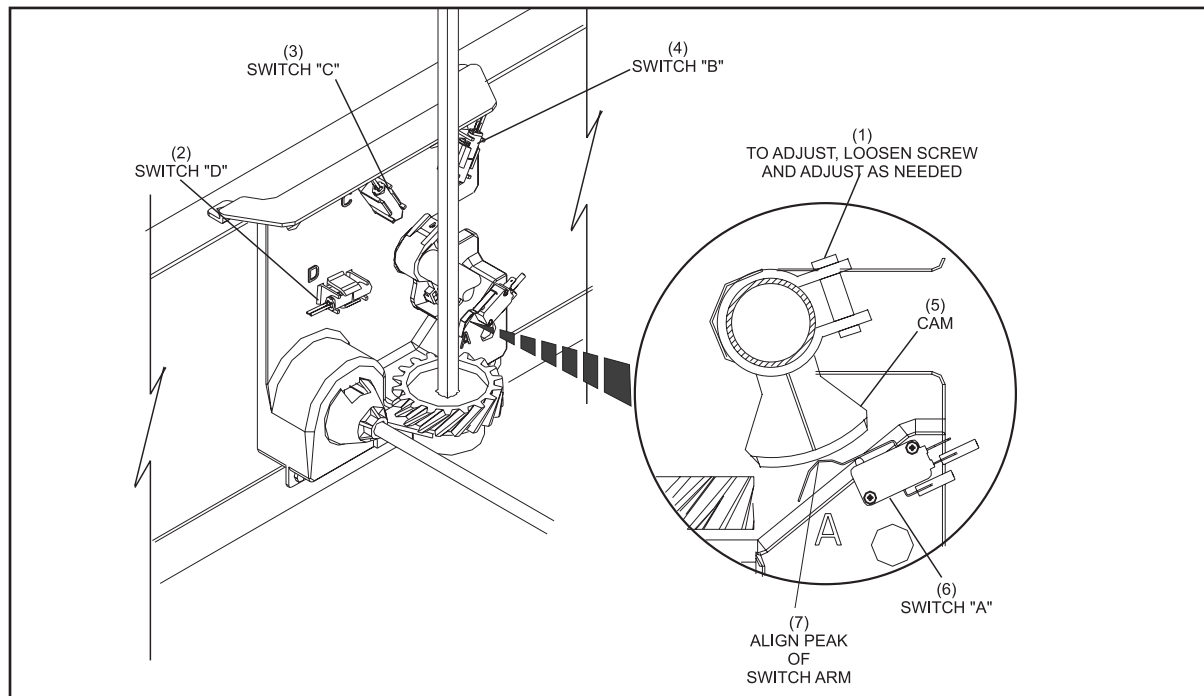
Figure 5-29. Cam Position
