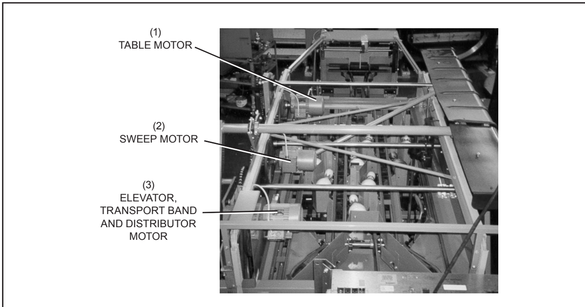
Figure 2-22. Pinsetter Motors
