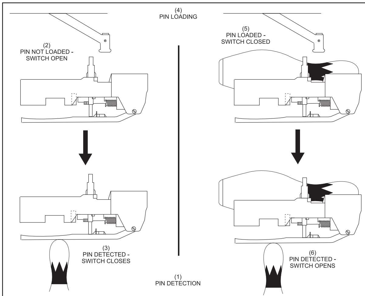
Figure I-15. Pin Detection
