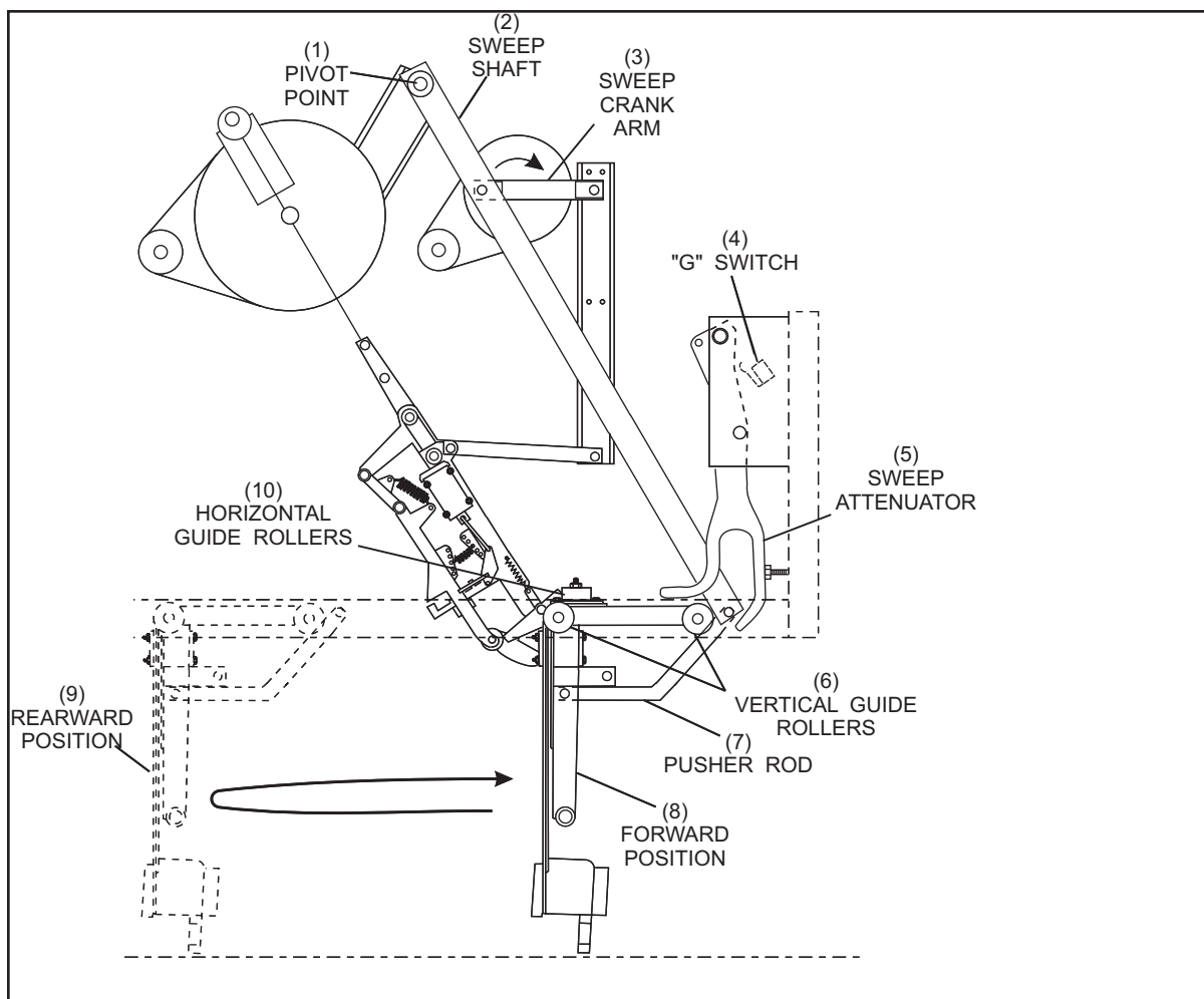
Figure 1-25. Sweep Motion.
