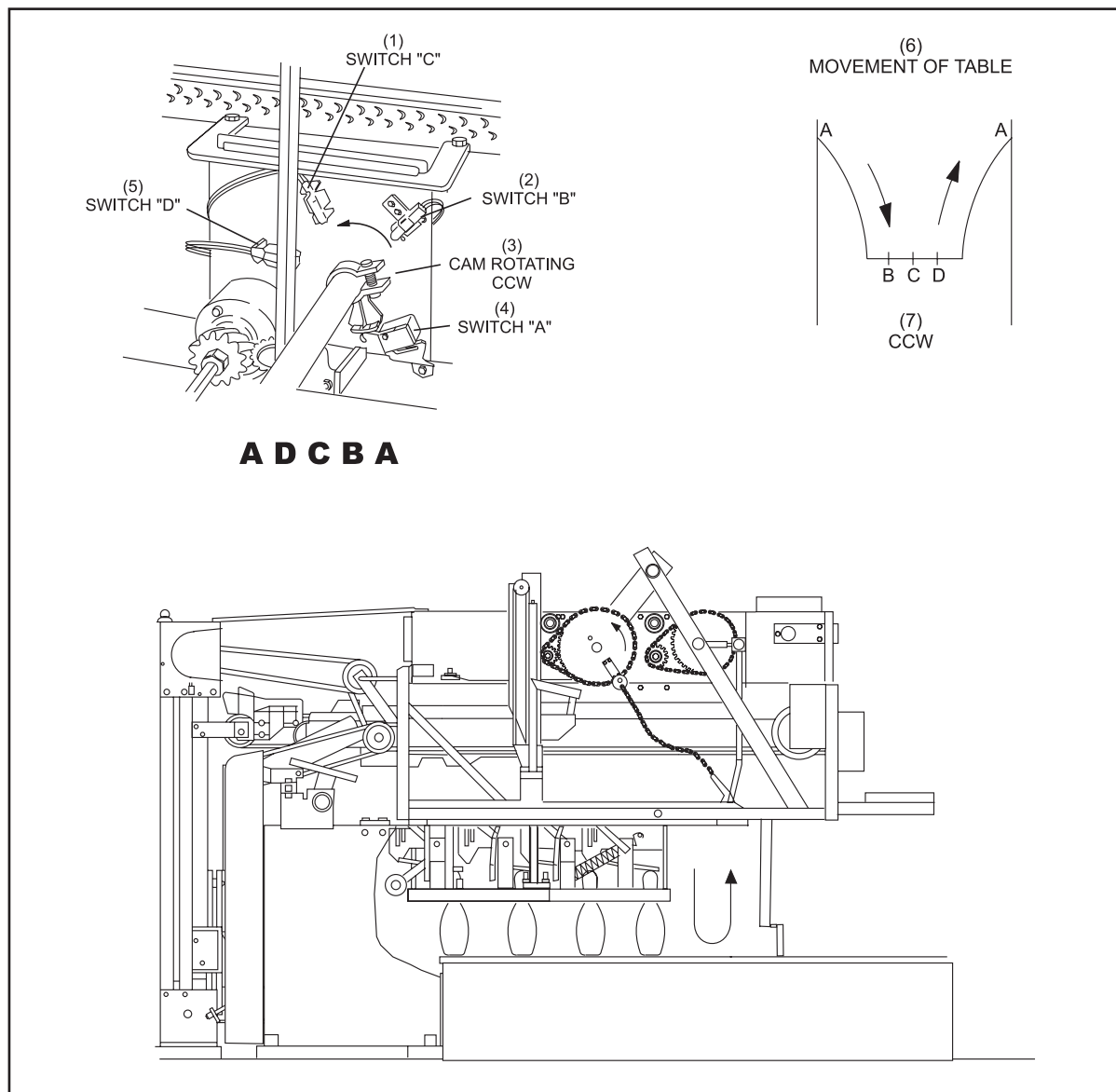
Figure 4-2. Detection Stroke
