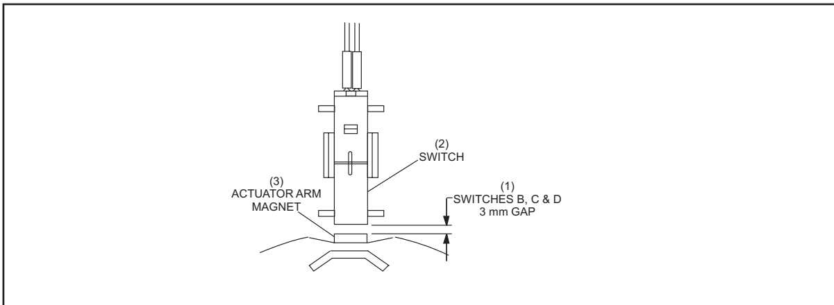
Figure 5-61. Adjusting switch Cluster
