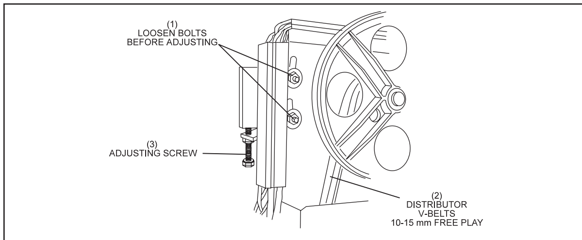
Figure 5-55. Adjusting Distributor V-Belts.
