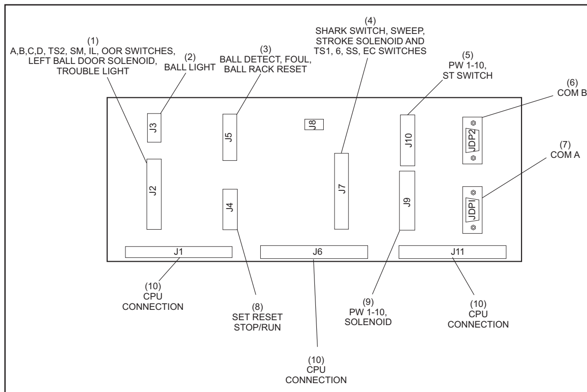
Figure 3-7. I/O PCB
