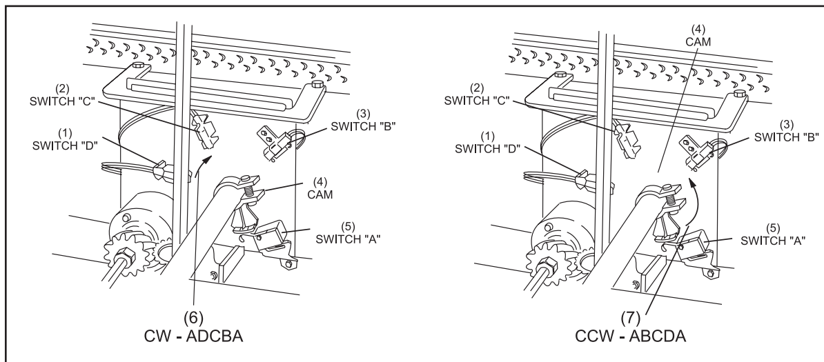
Figure 2-2. Switch Cluster
