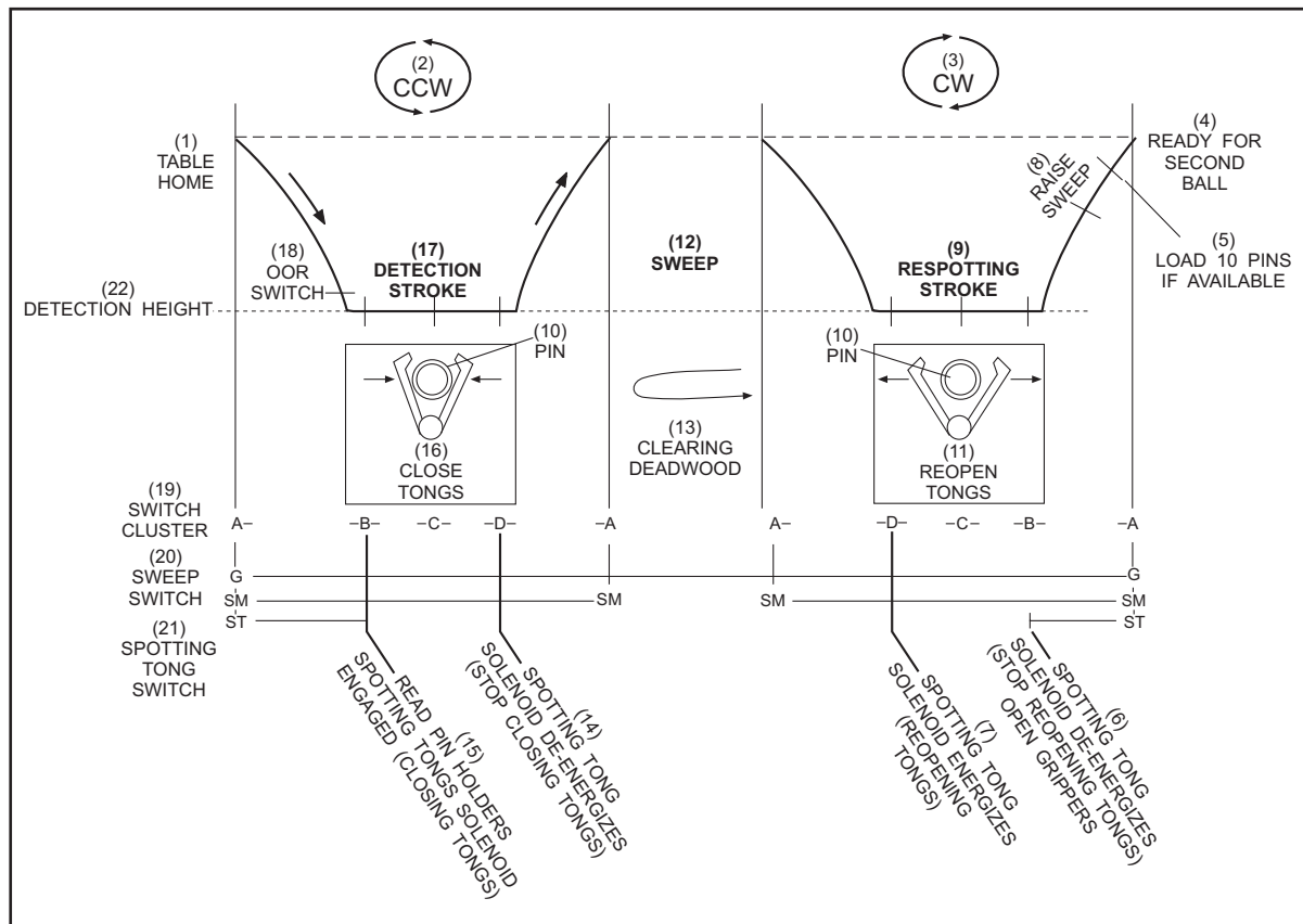
Figure 4-7. First Ball Standing Pins Cycle.
