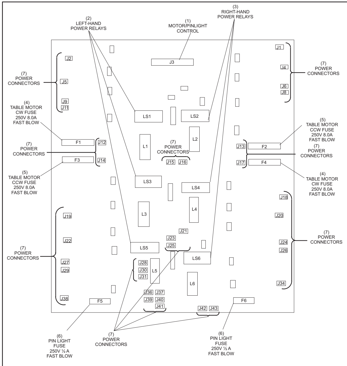
Figure 3-9. Nexgen Controller - High Voltage PCB
