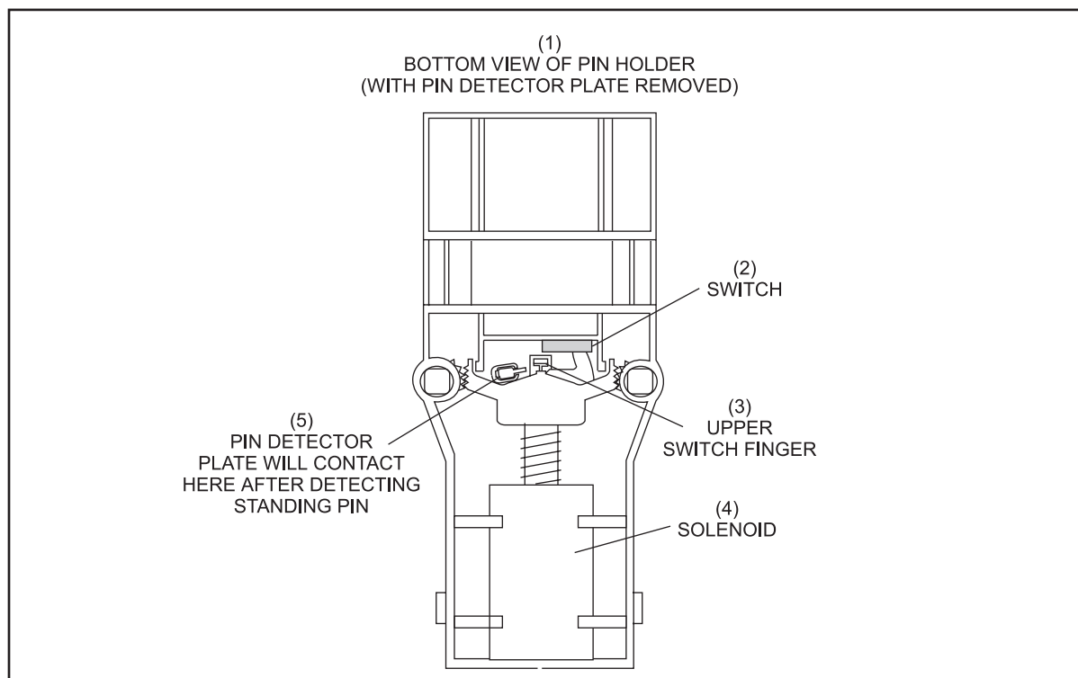
Figure 2-8. Pin Holder Detecting
