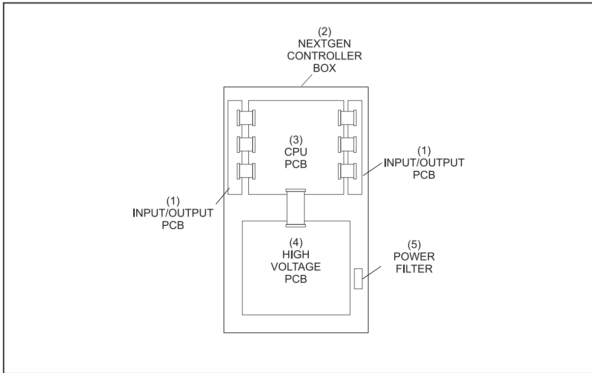
Figure 3-6. Nexgen Controller - Internal View
