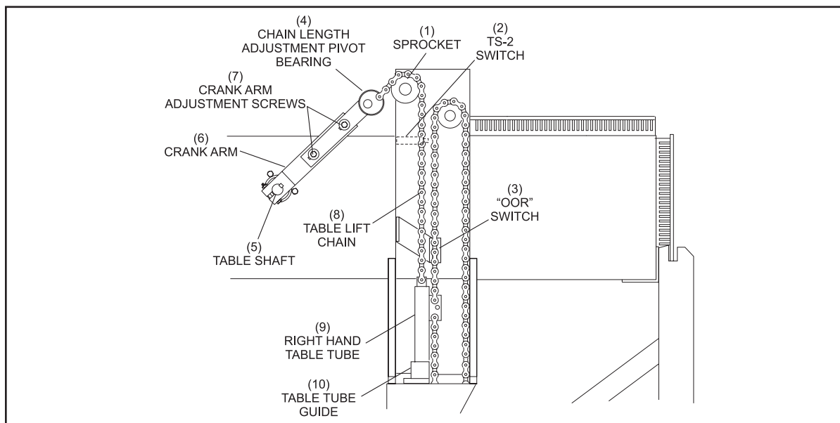
Figure 1-32. Right-Hand Guide Tower Assembly.
