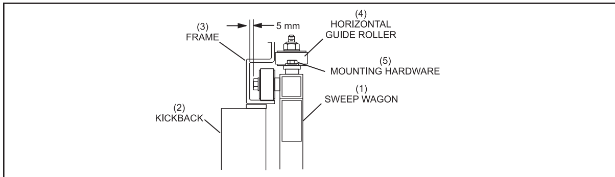
Figure 5-51. Sweep Wagon Roller Adjustment.
