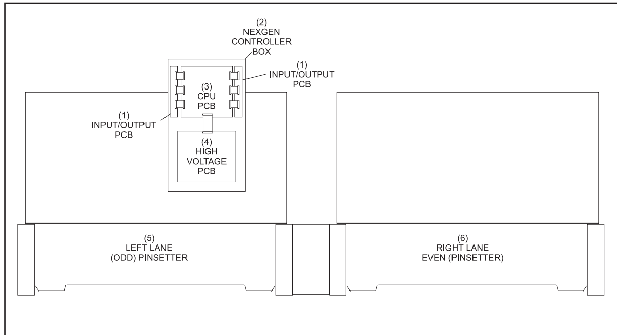
Figure 3-1. Nexgen Controller Box Layout.
