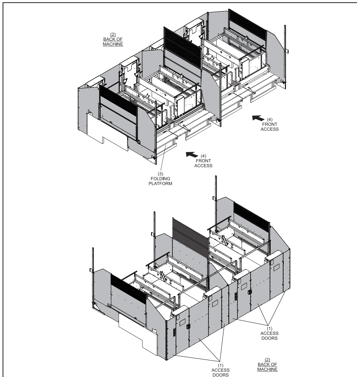
Pinsetter Access Points
