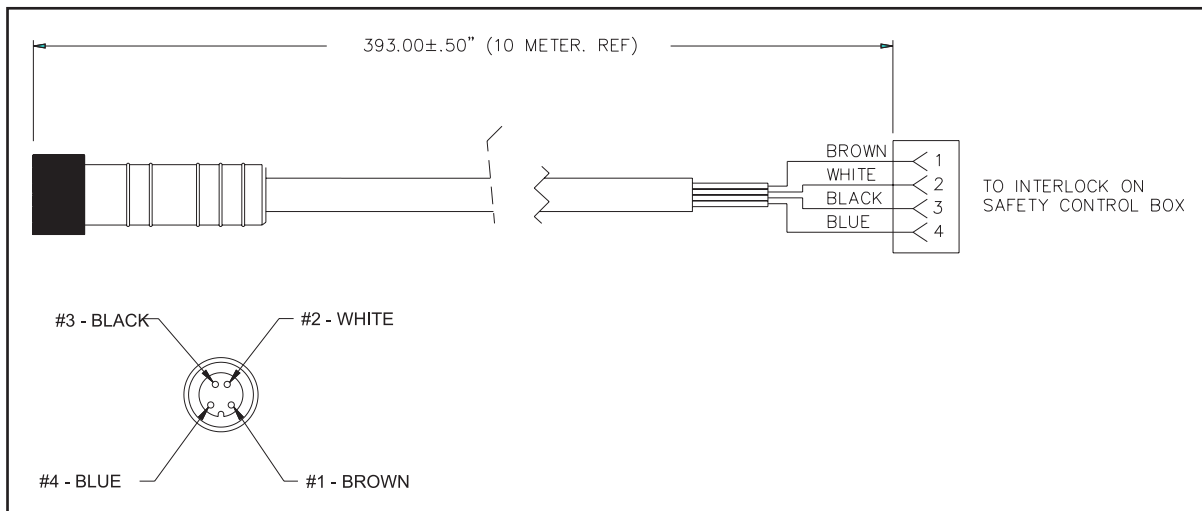
47-142881-000 - Masking Unit Interlock Cable
