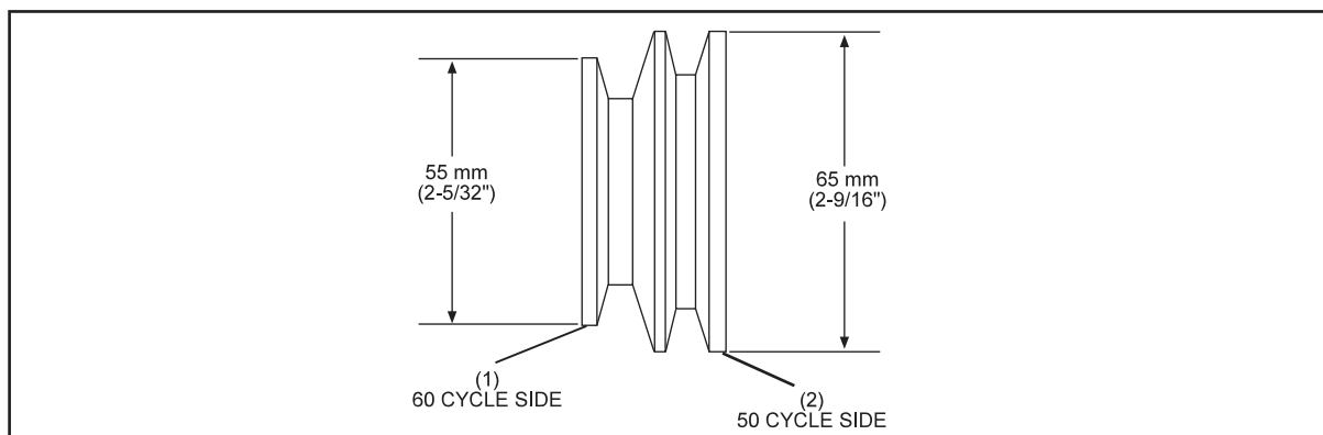
Figure 8-11. Dual Pulley.
