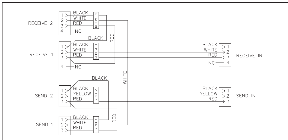
47-142875-000 - Photosensor Adapter Cable for Walkway with Obstruction
