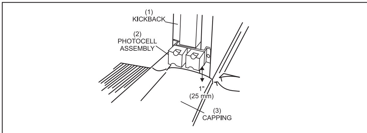
Figure 3-11. Ball Detect.
