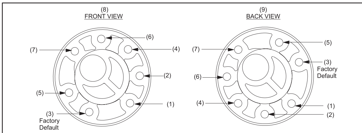
Figure 5-53. Sweep Board Pivot Bearing
