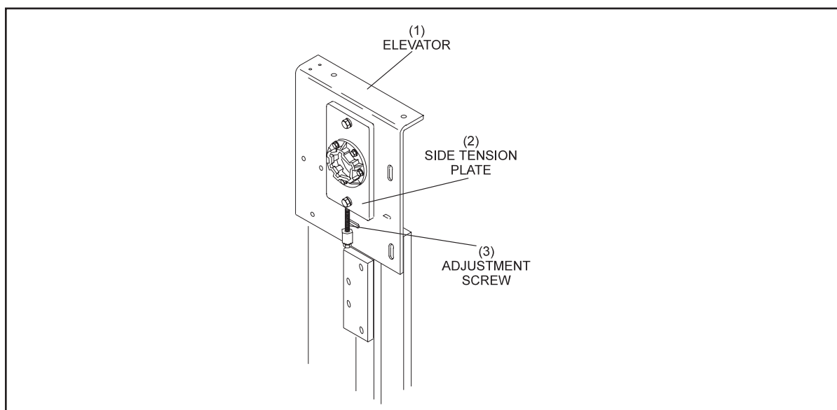
Figure 5-59. Elevator Chains.
