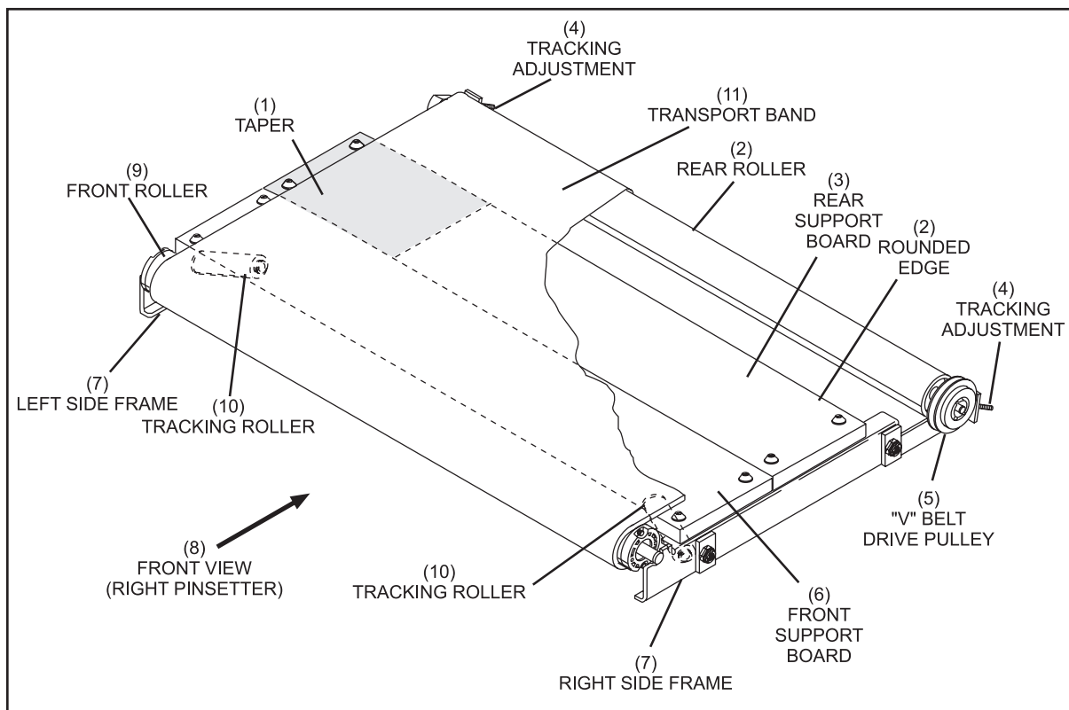
Figure 1-3. Transport Band.
