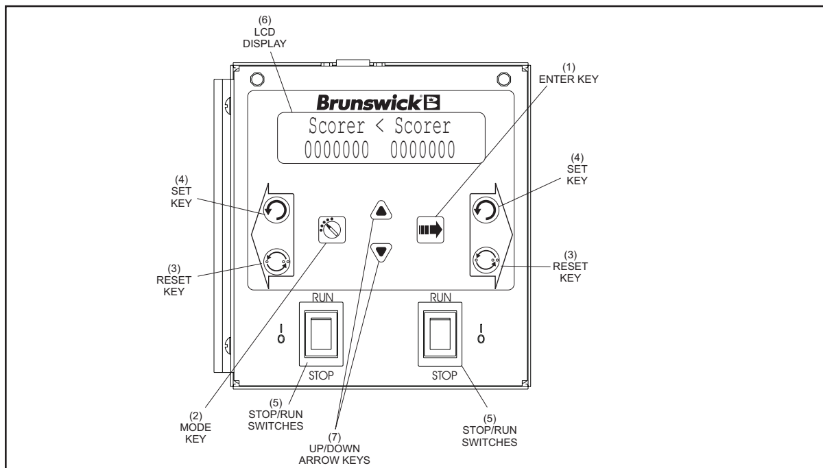
47-142750-4XX - Rear Display
