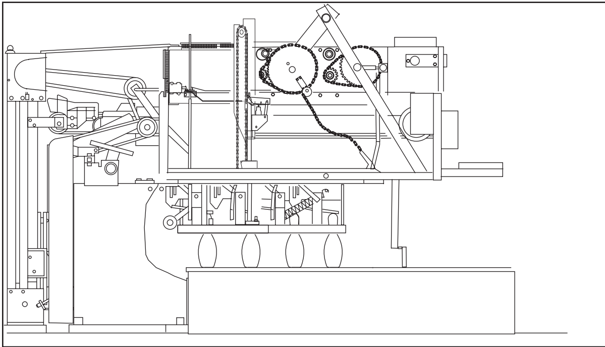
Figure 1-12. Detecting Pins
