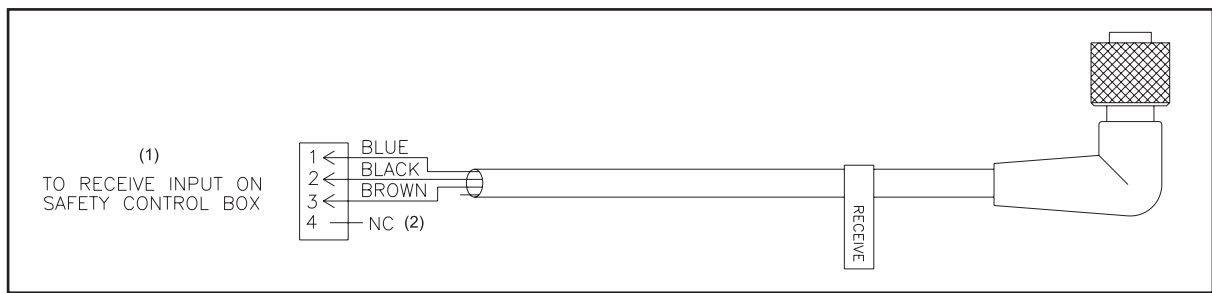
47-142863-000 - Photosensor Receiver cable Assembly
