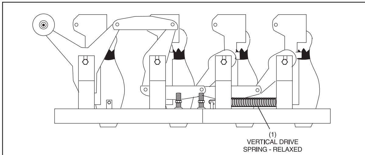
Figure 1-19. Setting New Pins Position.
