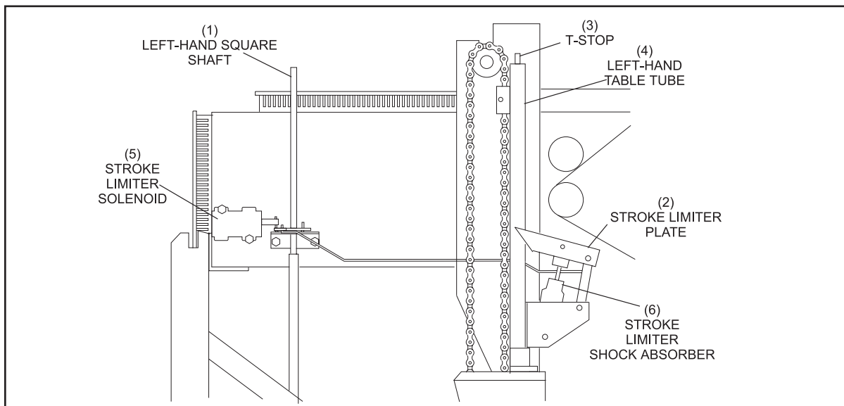
Figure 1-17. Left-Hand Table Rack with "T" Stop.
