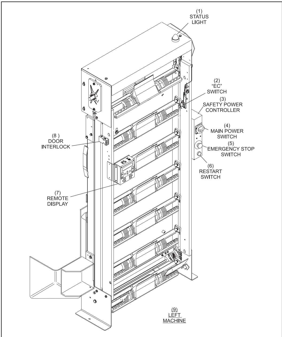
Figure 1-7. Elevator - Back View
