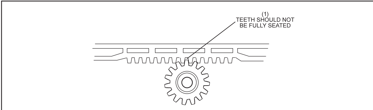
Figure 5-60. Adjusting for Proper Tooth Gap.
