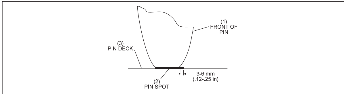
Figure 5-37. Proper Pin Position.
