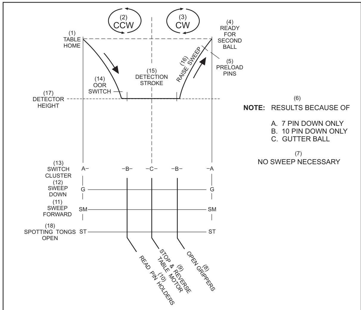
Figure 4-8. First Ball Short Cycle.
