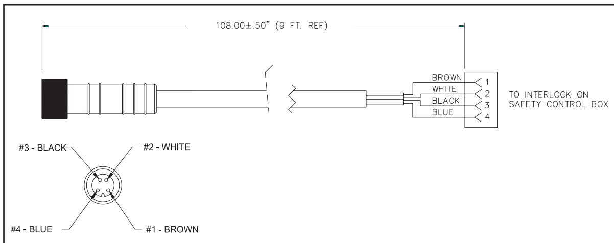
47-142880-000 - Rear Gate Interlock Cable
