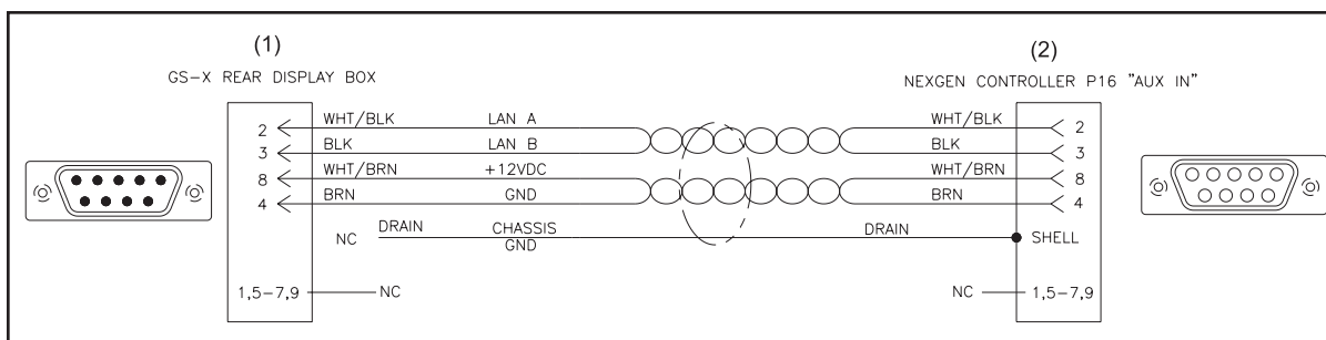
47-142761-000 - GS-X Display to Nexgen Cable Assembly (Pinsetter Series XXX - XXX)
