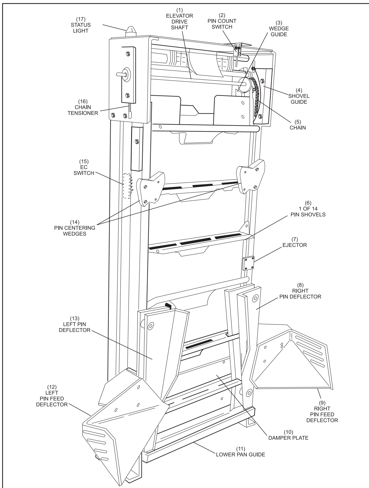
Figure I-6 . Elevator
