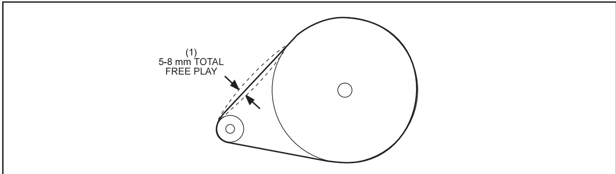
Figure 5-56. Sweep and Table Motor Chain Free Play.
