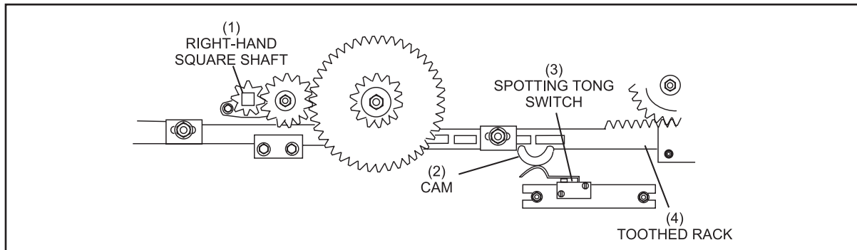
Figure 2-9. ST Switch with Tongs Open
