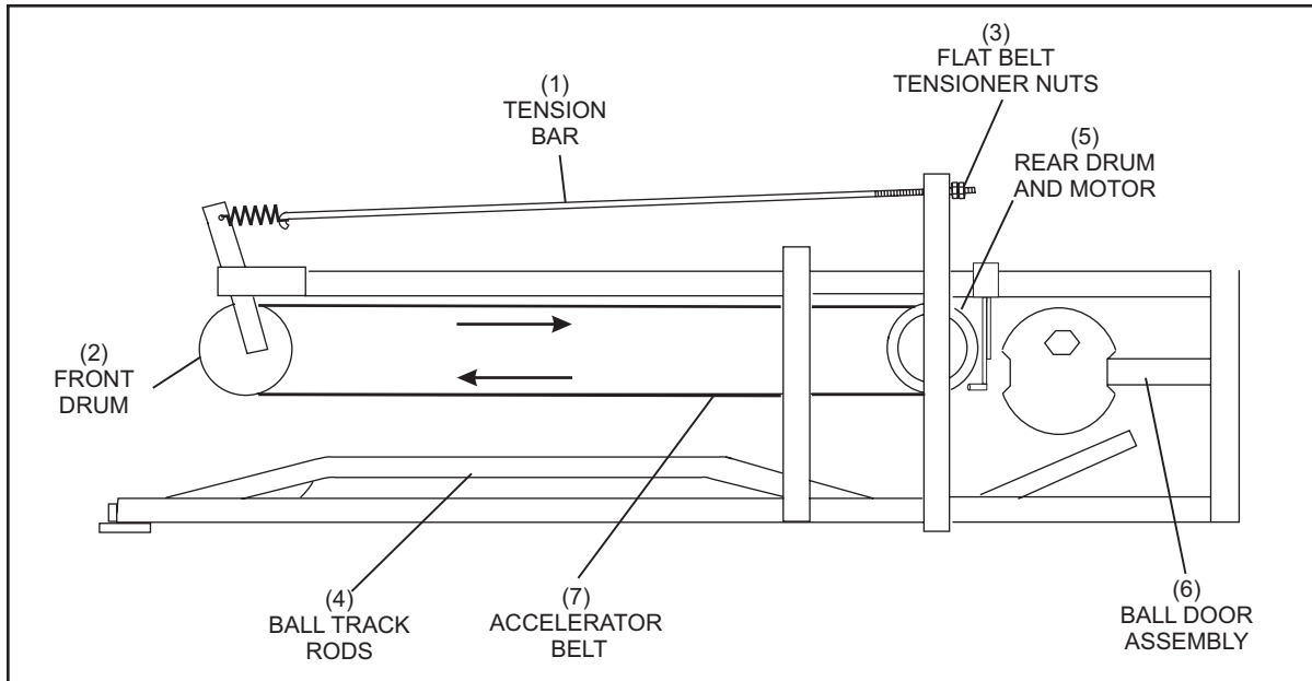
Figure 1-4. Ball Accelerator.
