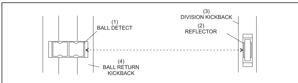
Figure 5-1. Ball Detect and Retroreflector.
