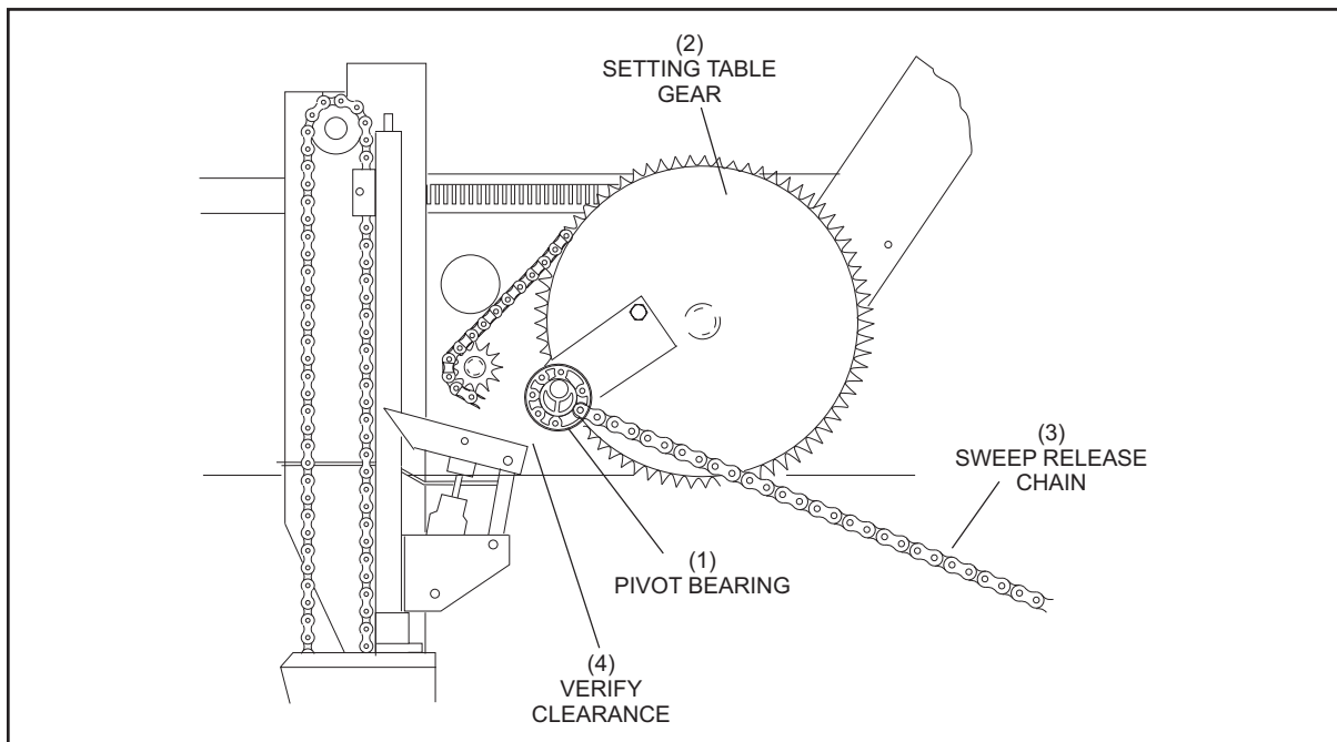
Figure 5-54. Verify Pivot Bearing Clearance
