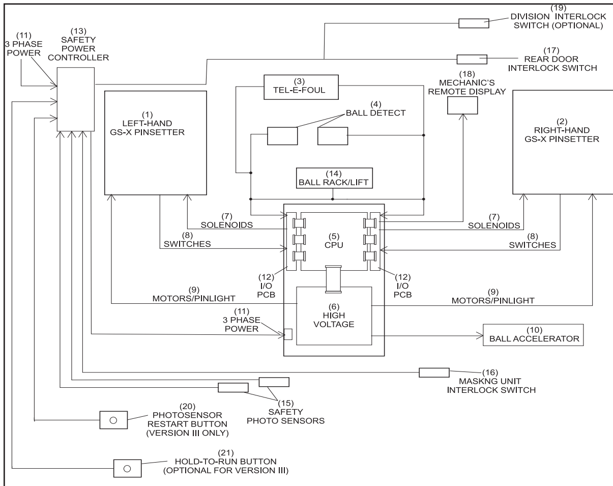
Figure 3-2. Pinsetter Block Diagram - Advanced (CE) Guard Packages
