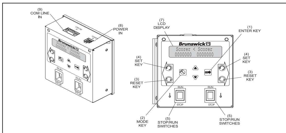
Figure 3-15 Remote Display
