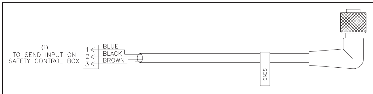
47-142864-000 - Photosensor Send Cable Assembly
