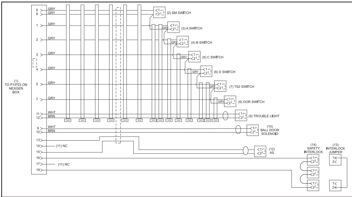
47-142730-000 - Right Side Function Cable Assembly (Revision B)
