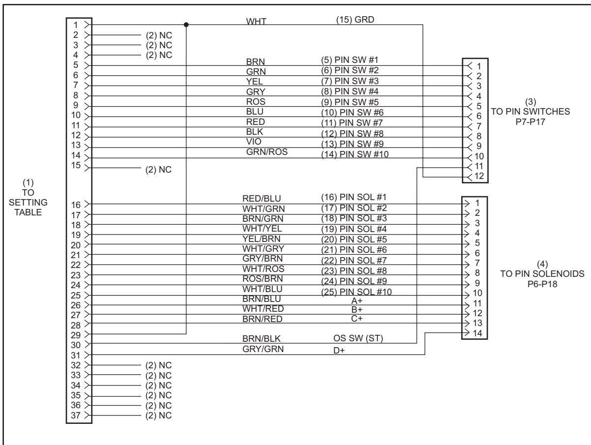
47-245421-004 - External Setting Table Cable Assembly
