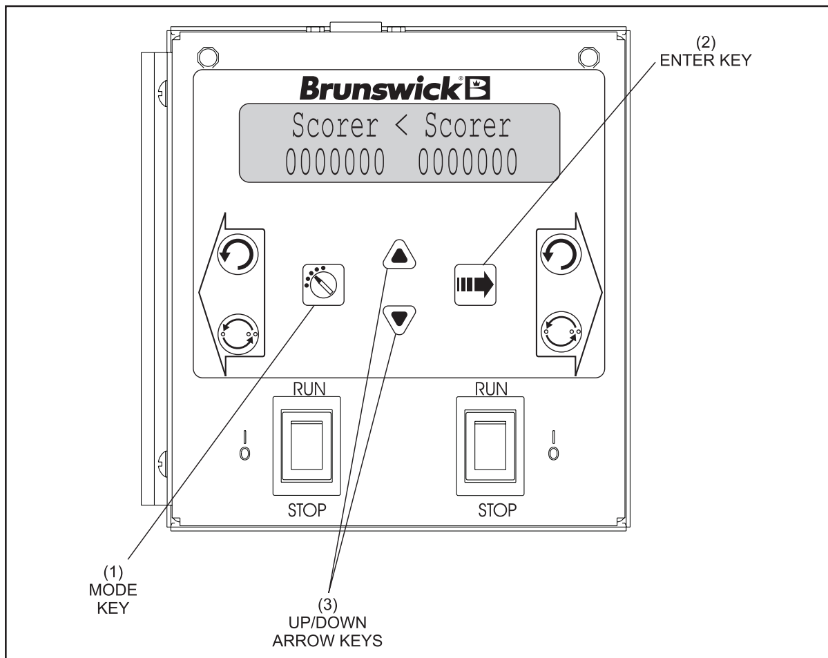
Figure 3-10. Nexgen Remote Display - LCD Panel
