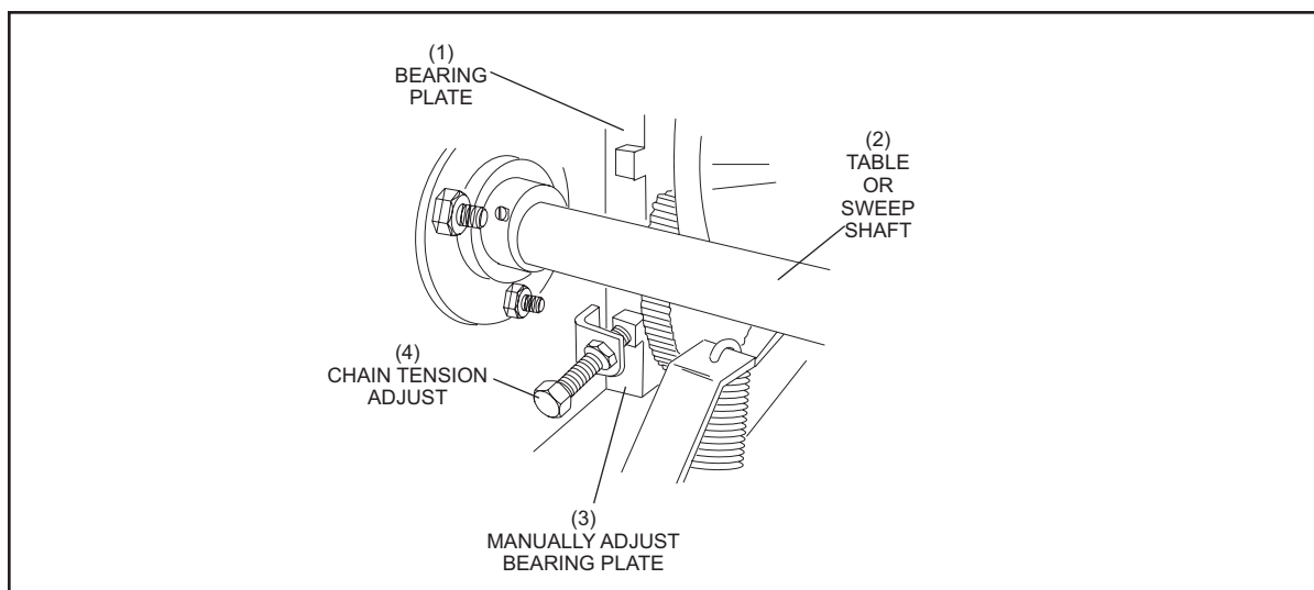
Figure 5-58. Chain Tension Adjuster.
