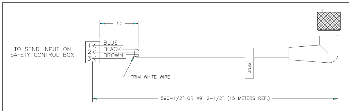
47-142865-000 - Photosensor Send Cable
