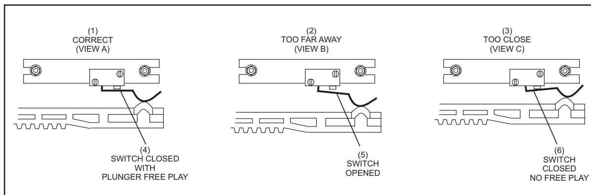
Figure 5-63. Spotting Tong Switches.
