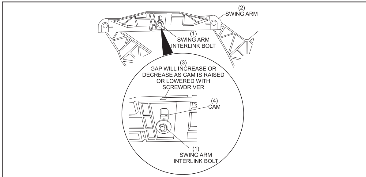
Figure 5-40. Swing Arm Adjustment.
