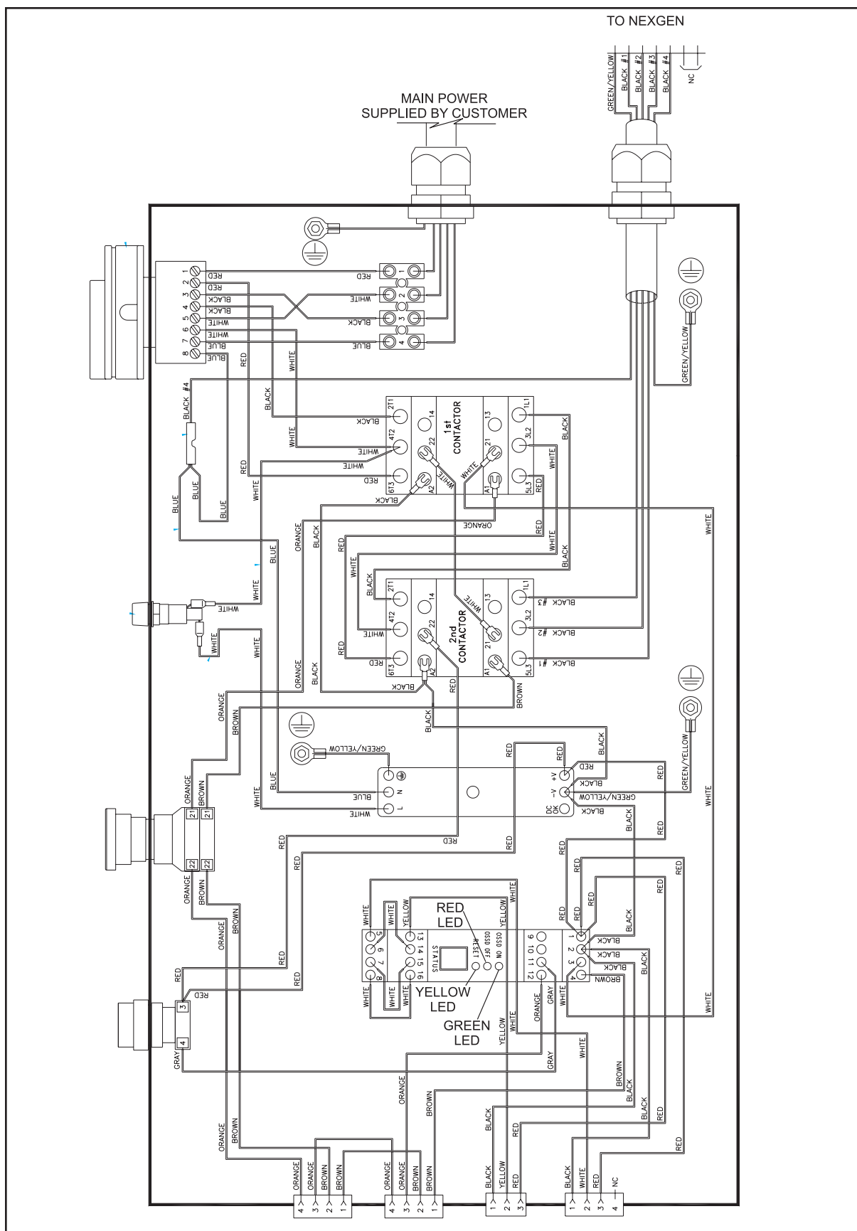
47-142834-000 - CE Safety Power Controller
