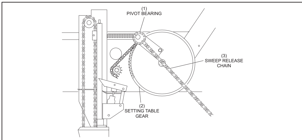
Figure 5-52. Sweep Board Height Adjustment.
