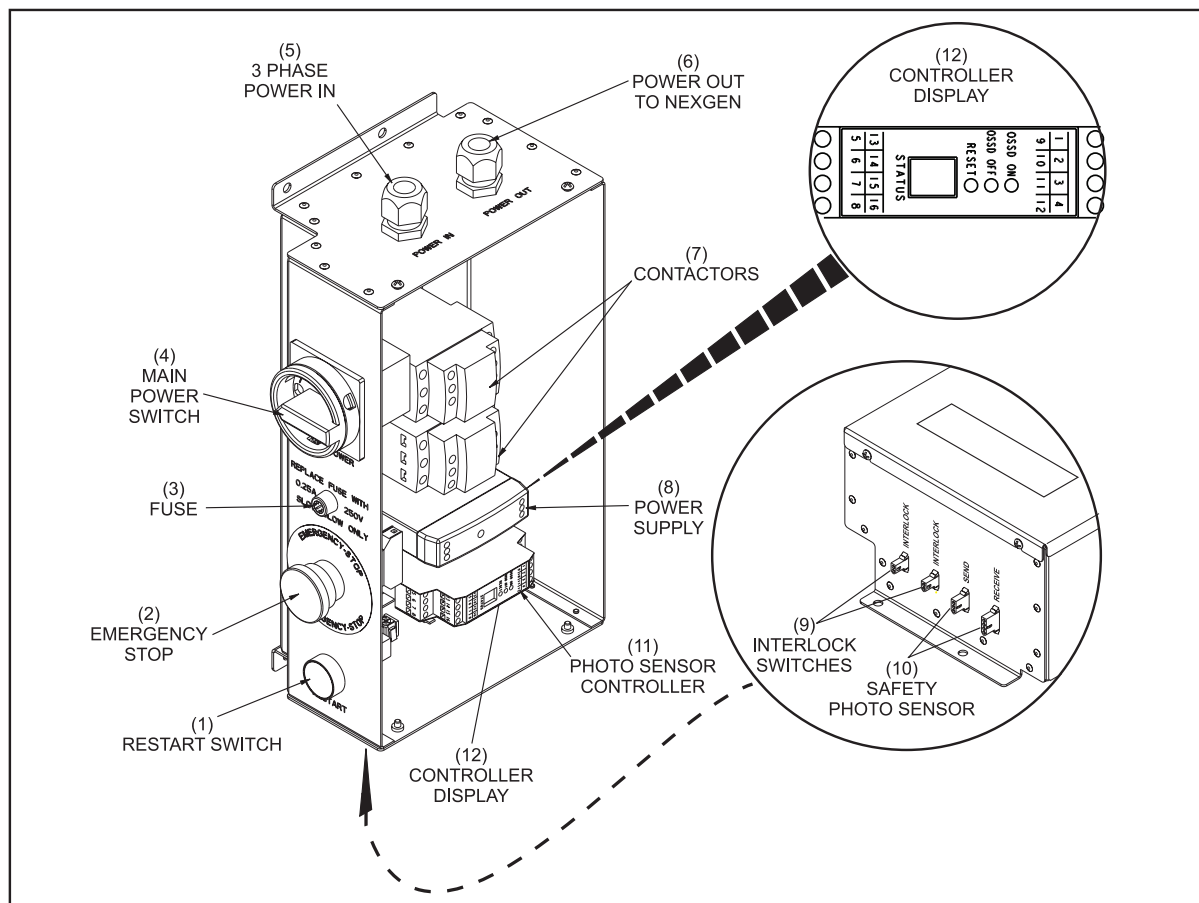
Figure 3-13. Safety Power Controller - Version I and II
