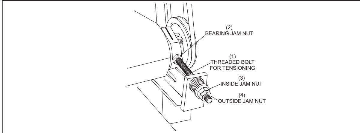
Figure 5-4. Jam Nut for Tensioning the Transport Band.
