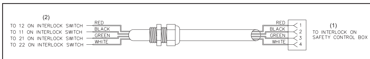
47-142861-000 - Masking Unit Interlock Cable Assembly
