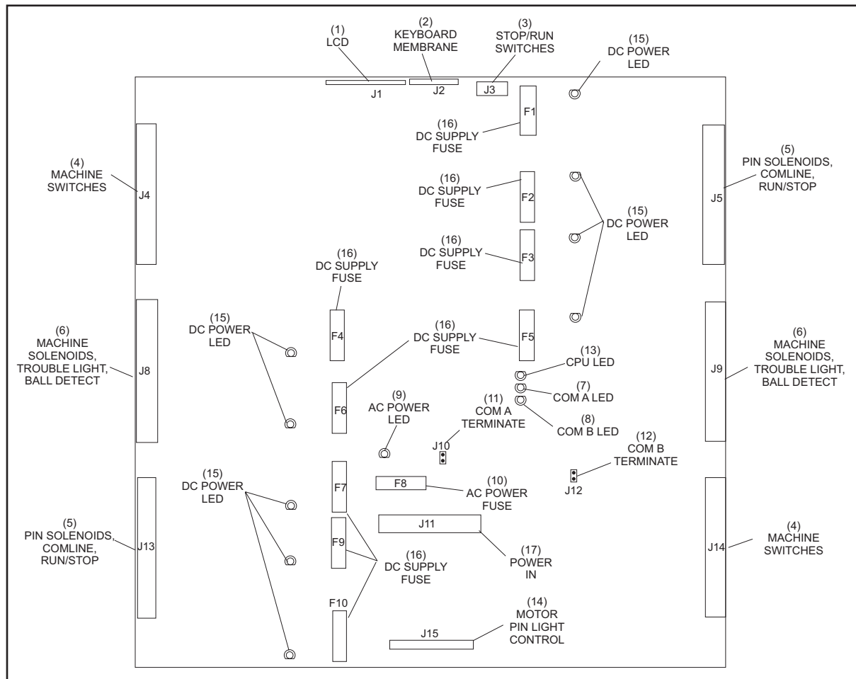
Figure 3-8. CPU PCB.
