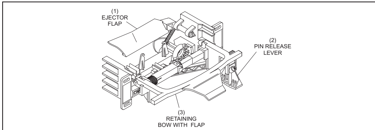
Figure 1-10. Pin Station
