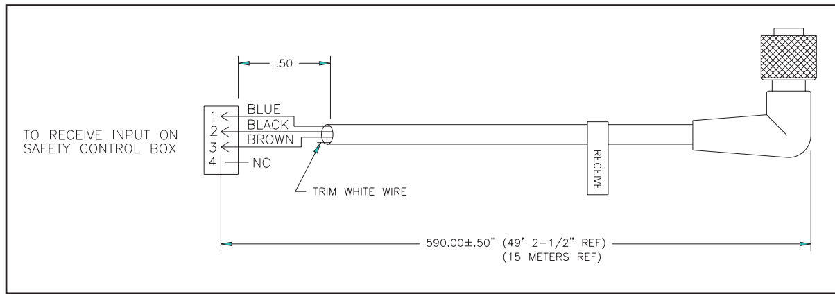
47-142874-000 - Photosensor Receive Cable
